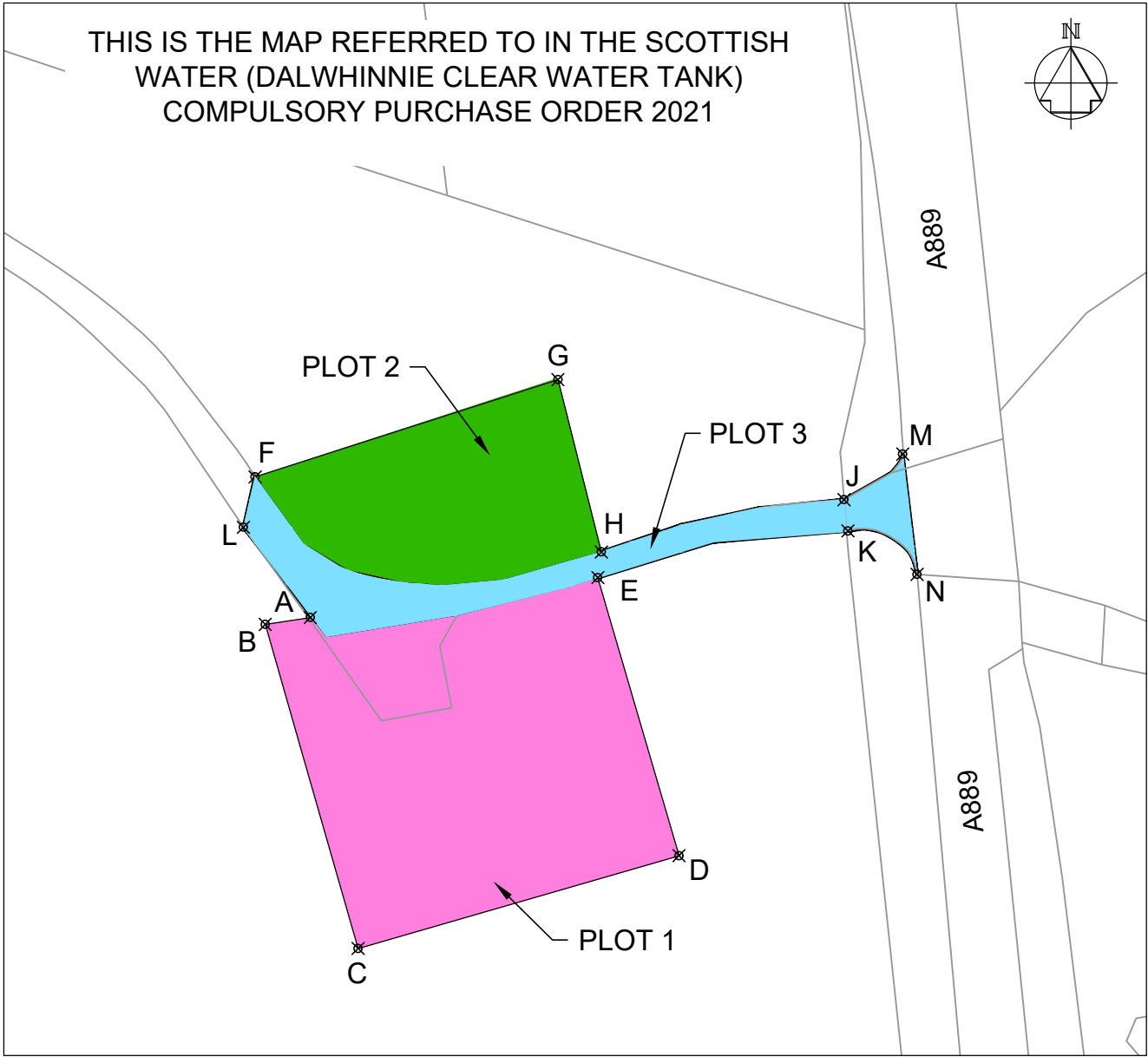
SITE LAYOUT Scale - 1:1250
